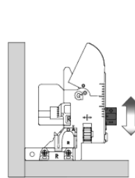
Front locking device
