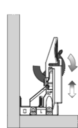
Eco front locking device
